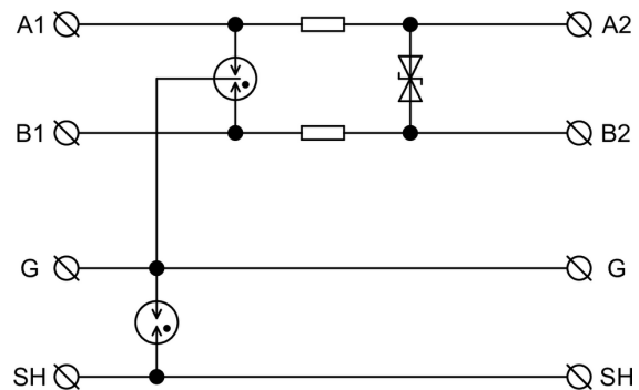
Internal diagram
